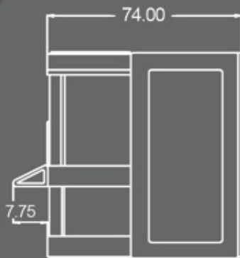
SIDE ELEVATION
